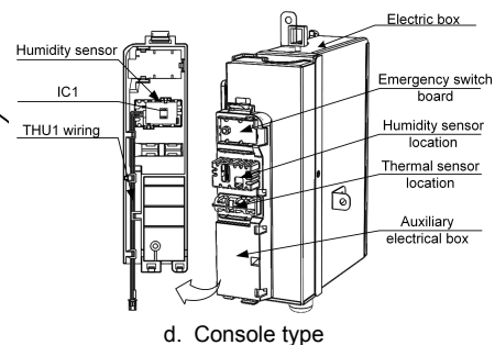
d. Console type
